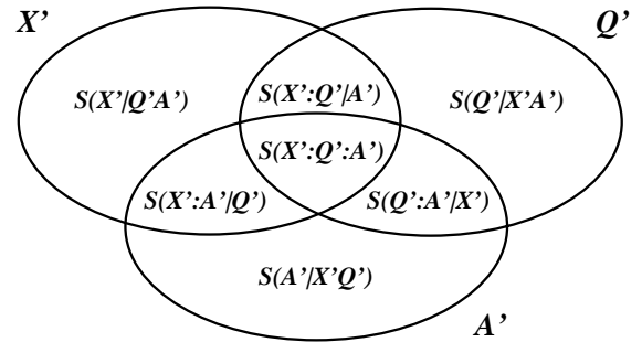
FIG. 2. Venn diagram summarizing the relation between entropies (defined in the text) after measurement in the system X'Q'A' .
