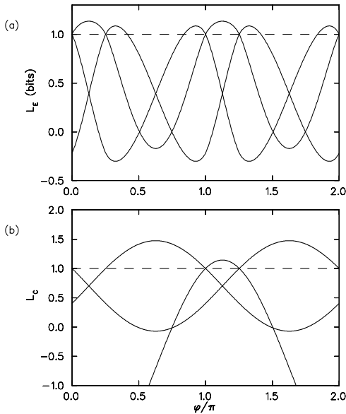
FIG. 2. (a) Left-hand side L_E of entropic Bell inequalities Eqs. (17-19) for EPR Bell-measurements with \theta = \pi/3.958 . The inequalities are violated if L_E > 1 ; (b) Left-hand side L_C of conventional inequalities Eqs. (4-6) at the same angle.
