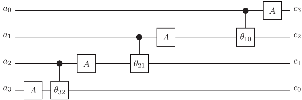
Figure 1: QFT network operating on a four-bit register. The phases \theta_{jk} that appear in the operations B_{jk} are related to the “distance” of the qubits ( j - k ) and are given by \theta_{jk} = \pi/2^{j-k} . The network should be read from the left to the right: first the gate A is effected on the qubit a_3 , then B(\phi_{32}) on a_2 and a_3 , and so on.
