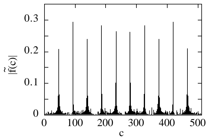
m=1 (Hadamard)
