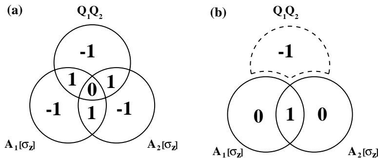
Fig. 5. (a) Quantum entropy diagram for the EPR measurement of same spin-projections: e.g., A_1 and A_2 both measure \sigma_z . (b) reduced diagram obtained by tracing over the quantum states Q_1 and Q_2 .
